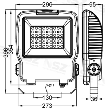
ZY-2071SMD 100/120W
