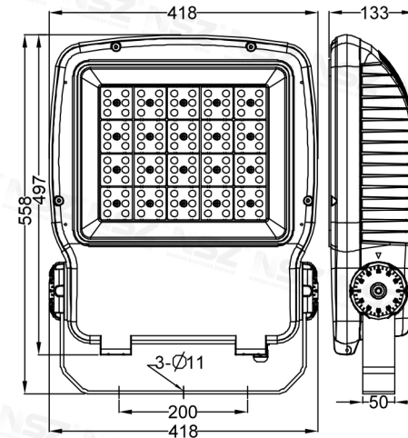
ZY-2071SMD 300/400W
