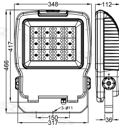
ZY-2071SMD 150/200W
