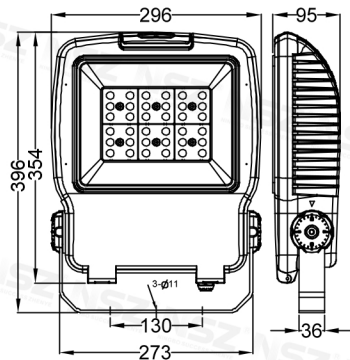
ZY-2071SMD 80W
